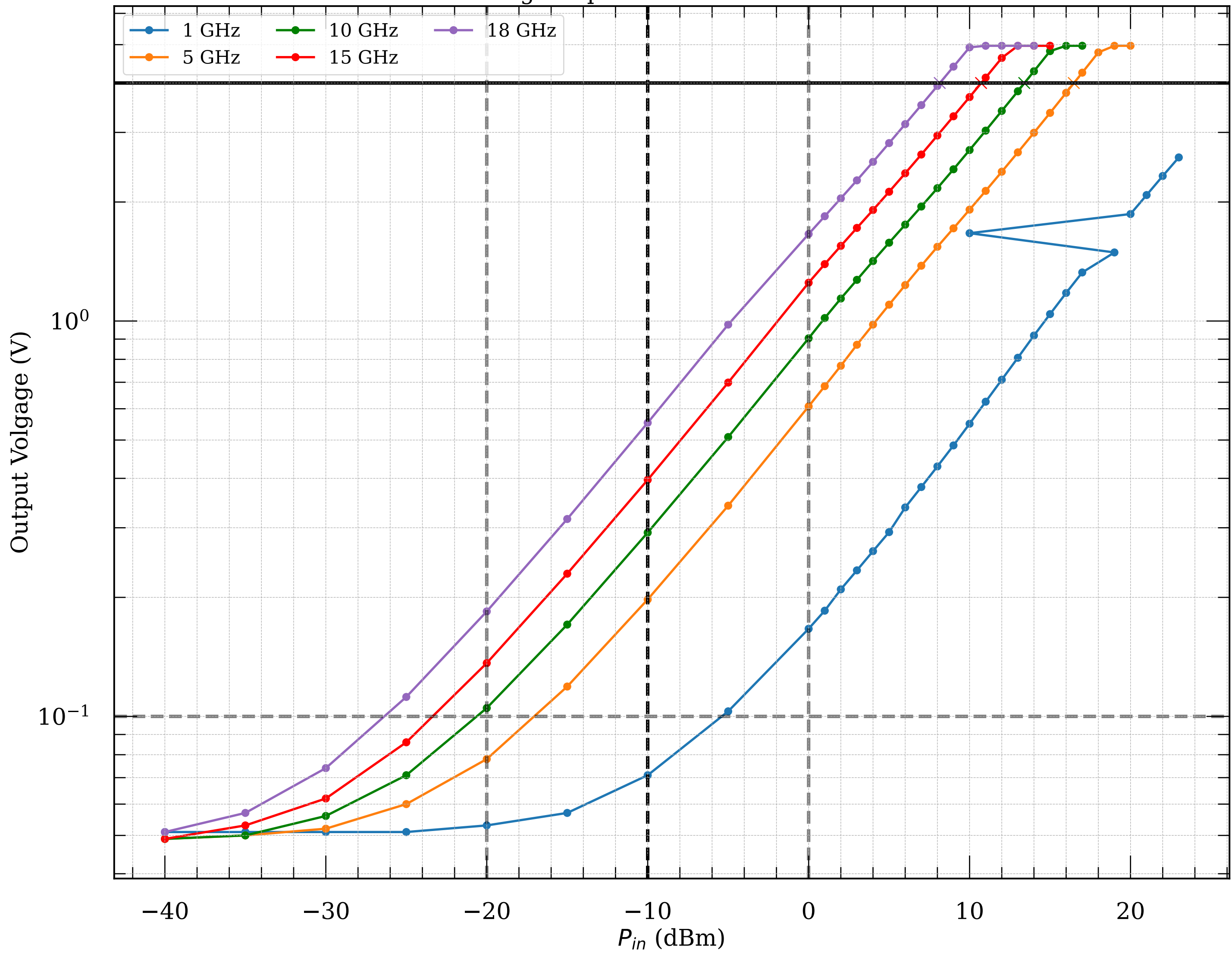
Measured voltage-to-power curve of detector module063
